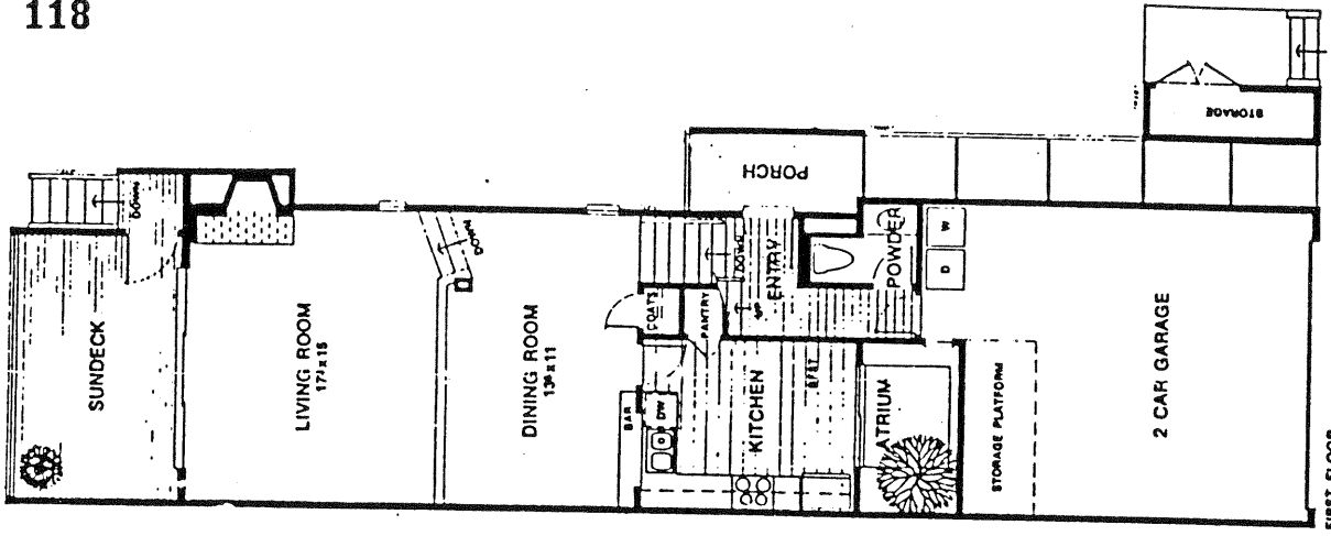
DEL MAR WOODS TOWNHOMES Model: PLAN A-1 Area: 1143 B/T Code: DWT Approximate SQ/FT: 1468
